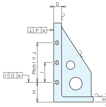
T-slot dimension
