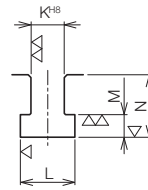
T-slot dimension
