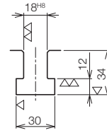
T-slot dimension
